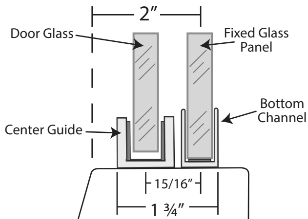
Barn Door Vertical Cross Section
