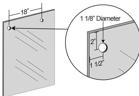
Fixed Panel Hole Specifications
