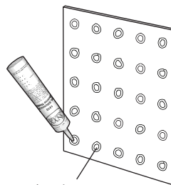
Silicone Application about 8" apart Can be applied to panel or walls
