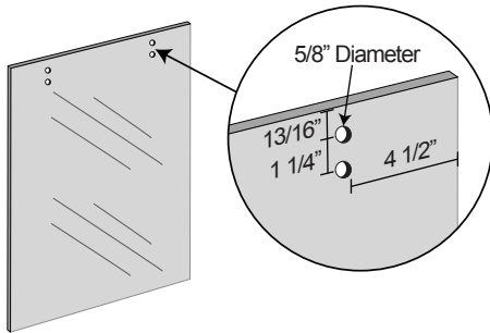
Door Panel Hole Specifications
