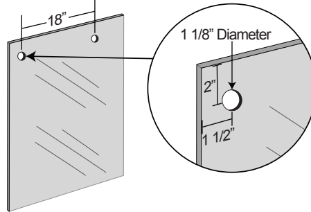
Fixed Panel Hole Specifications
