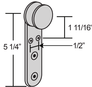
Roller Plate
