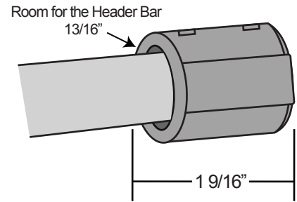
Bar Mount Blocks
