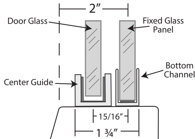
Barn Door Vertical Cross Section
