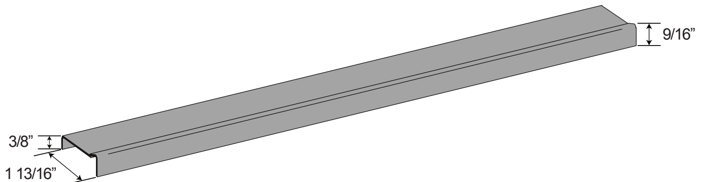
Curb Track
